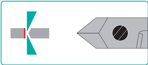
Without bevel
