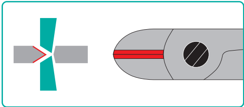
With bevel
